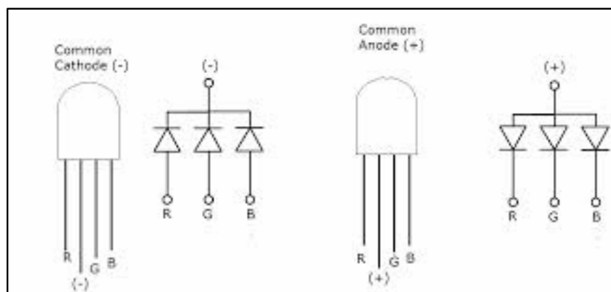
Figure 3-5 Circuit Diagram of RGB LEDs Permission Pending
