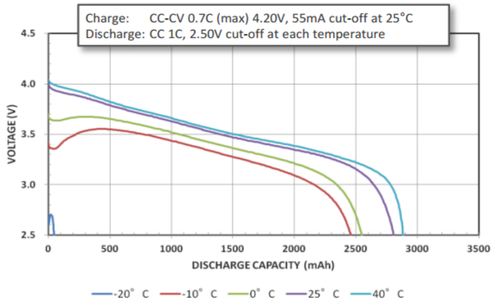
Figure 3-3 Battery Discharge Characteristics Permission Pending
