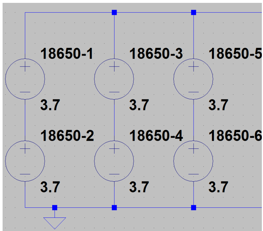
Figure 4-3 Panasonic 18650 Battery Configuration
