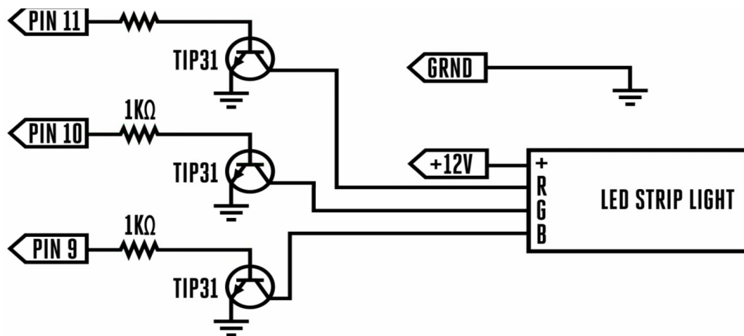
Figure 3-1 Example RGB Wiring Permission Pending
