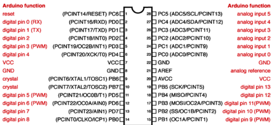
Figure 4-5 [30] Pin Layout of ATmega328P
