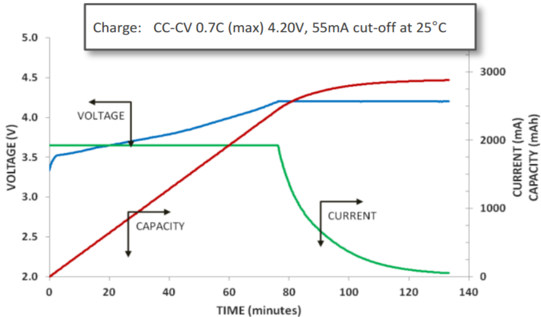
Figure 3-4 Ideal Charging Characteristics for Panasonic 18650 Battery Cells Permission Pending
