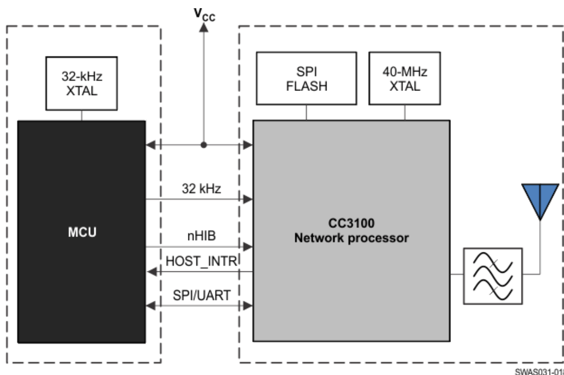
Figure 3-6 Example CC3100 Wiring Format Suggested by Texas Instruments Permission Pending
