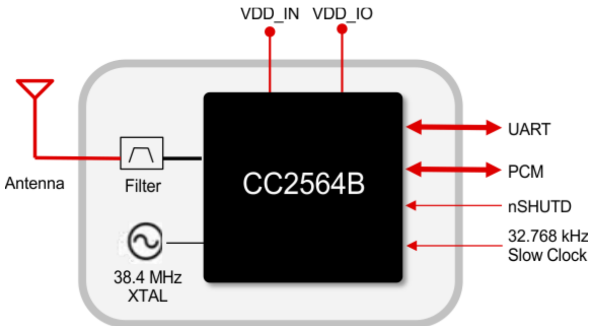
Figure 3-9 Wiring Format of CC2564B 4.1 Bluetooth Module Permission Pending
