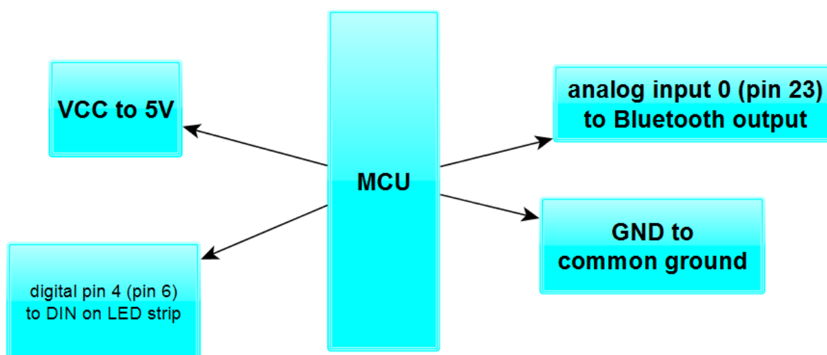
Figure 4-6 MCU Perspective of System
